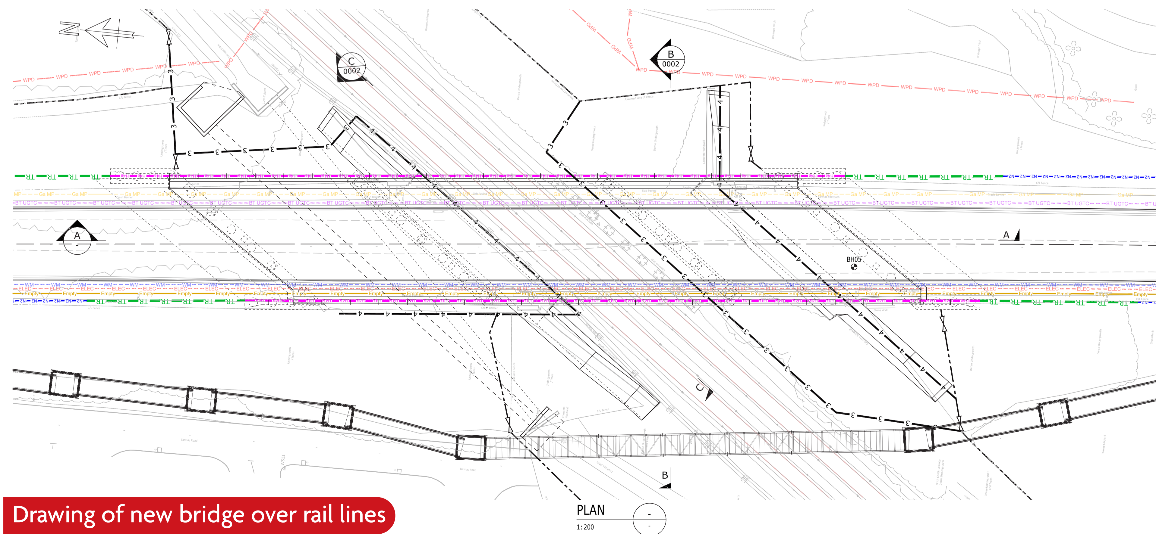
Drawing showing new bridge's foundations
